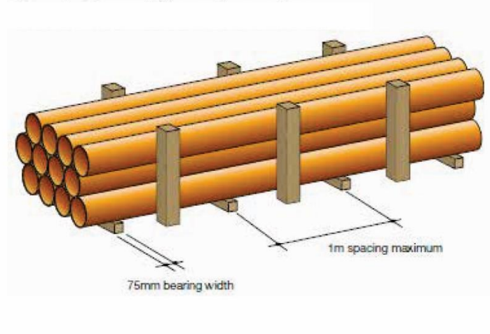
Figure 14: Storage of loose pipes on bearers
